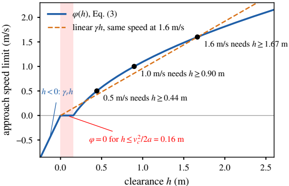
(a) barrier for static rows ( a = 1.47 \text{ m/s}^2 , T_d = 0.40 \text{ s} )
