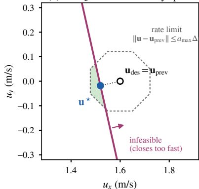
(b) one QP solve in velocity space
